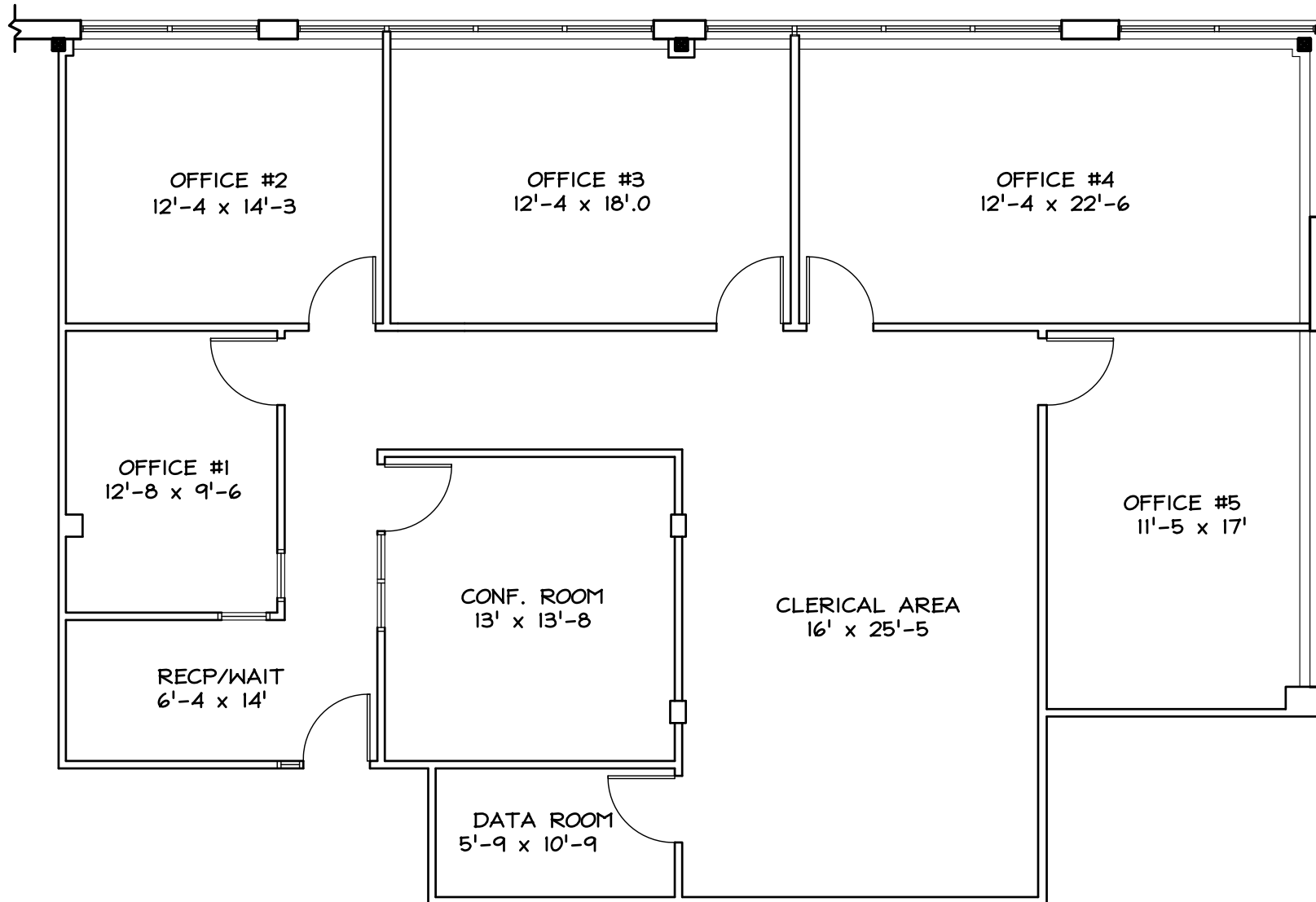
○ FLOOR PLAN - 2,371 RSF SUITE 102
